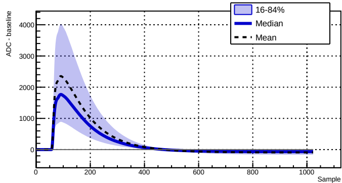
Run 039510 - Channel 2080 - 33062 waveforms
