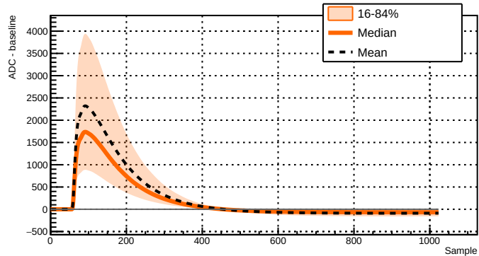
Run 039510 - Channel 2081 - 32656 waveforms
