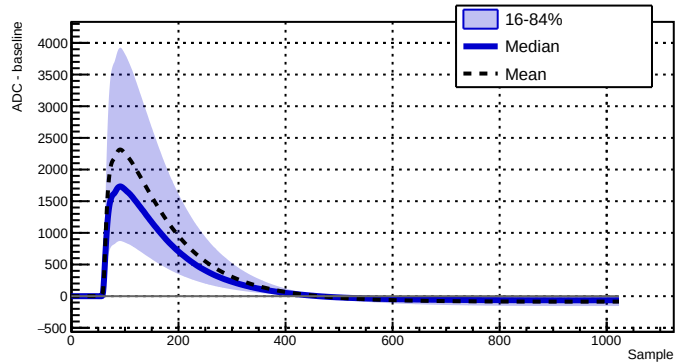
Run 039511 - Channel 2080 - 32676 waveforms
