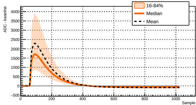
Run 039511 - Channel 2081 - 32269 waveforms
