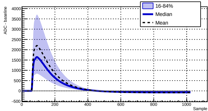
Run 039514 - Channel 2080 - 29773 waveforms
