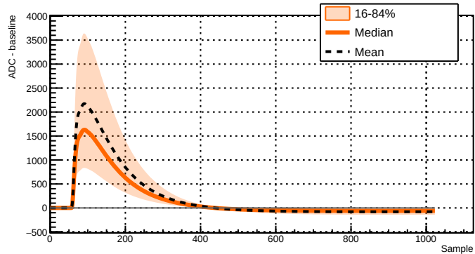
Run 039514 - Channel 2081 - 29335 waveforms
