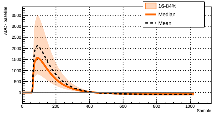
Run 039515 - Channel 2081 - 27884 waveforms
