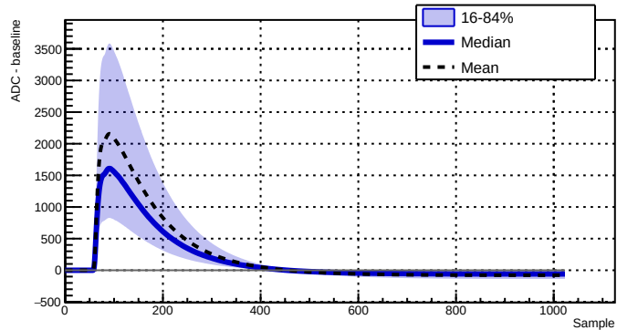
Run 039515 - Channel 2080 - 28261 waveforms
