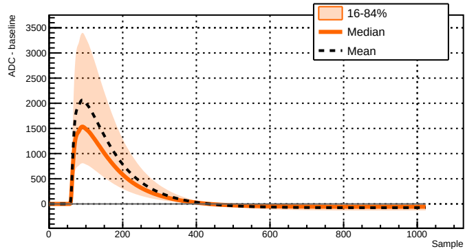
Run 039516 - Channel 2081 - 27077 waveforms
