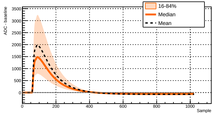
Run 039518 - Channel 2081 - 26633 waveforms
