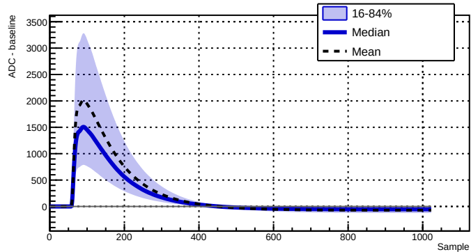
Run 039518 - Channel 2080 - 26982 waveforms
