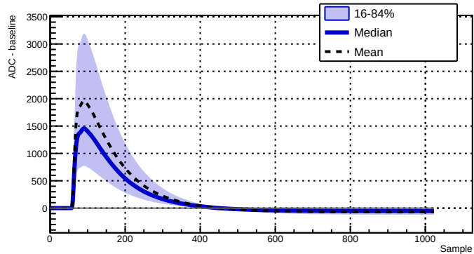
Run 039519 - Channel 2080 - 26376 waveforms
