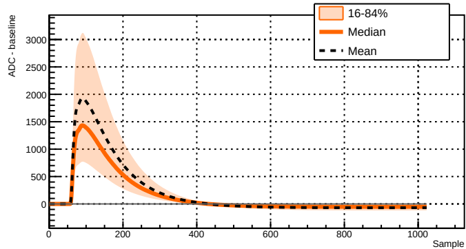
Run 039519 - Channel 2081 - 26017 waveforms
