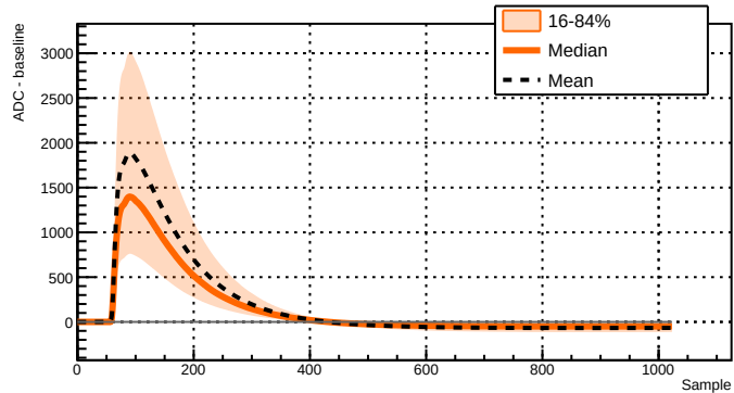
Run 039521 - Channel 2081 - 25156 waveforms
