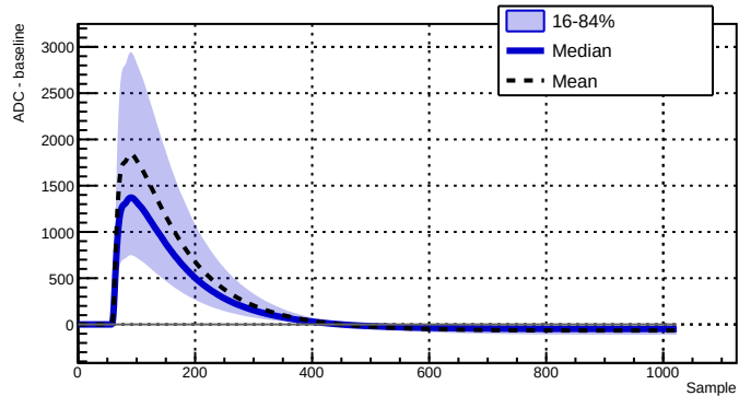
Run 039523 - Channel 2080 - 24599 waveforms
