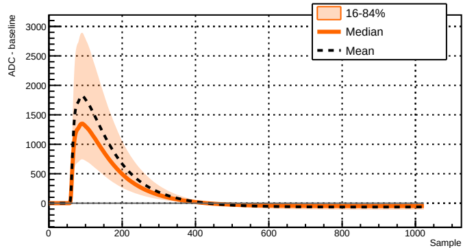
Run 039523 - Channel 2081 - 24235 waveforms
