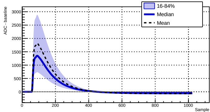
Run 039525 - Channel 2080 - 23976 waveforms
