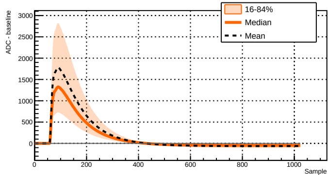
Run 039525 - Channel 2081 - 23653 waveforms
