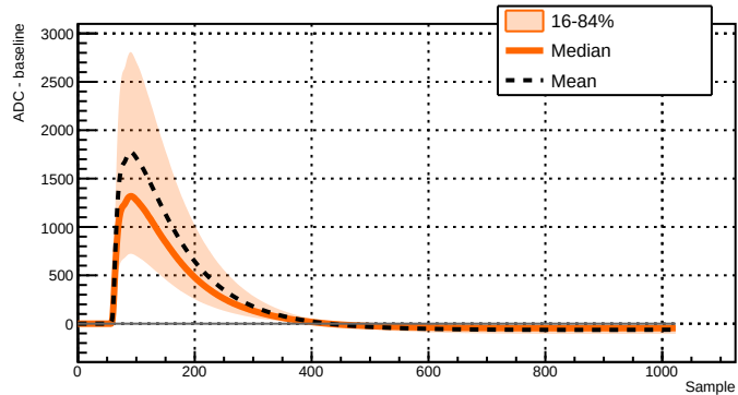
Run 039526 - Channel 2081 - 23392 waveforms
