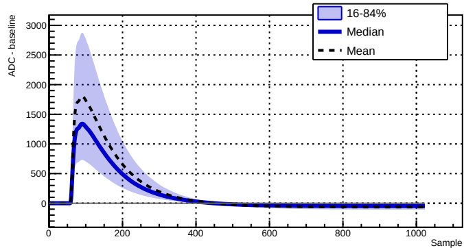
Run 039526 - Channel 2080 - 23722 waveforms
