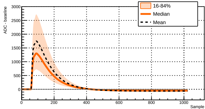
Run 039527 - Channel 2081 - 22847 waveforms
