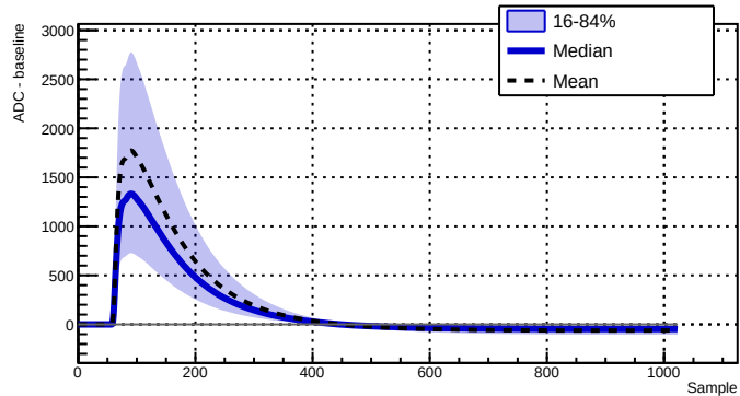
Run 039527 - Channel 2080 - 23342 waveforms
