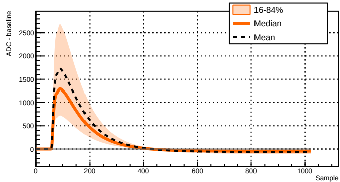
Run 039528 - Channel 2081 - 22550 waveforms
