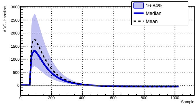
Run 039528 - Channel 2080 - 23009 waveforms
