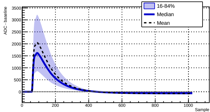
Run 039501 - Channel 2080 - 17130 waveforms
