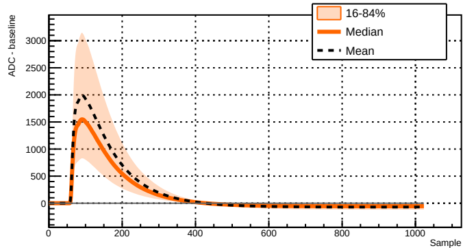
Run 039501 - Channel 2081 - 17615 waveforms
