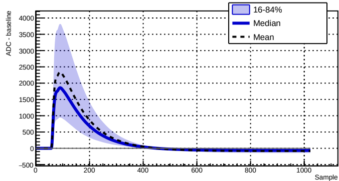
Run 039506 - Channel 2080 - 20987 waveforms
