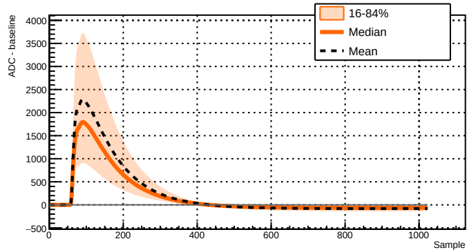
Run 039506 - Channel 2081 - 21390 waveforms
