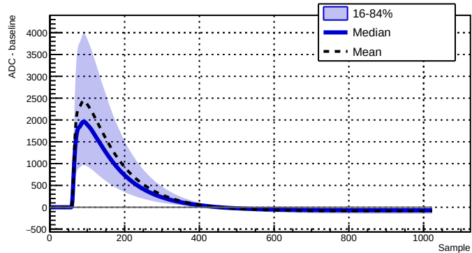
Run 039507 - Channel 2080 - 22378 waveforms
