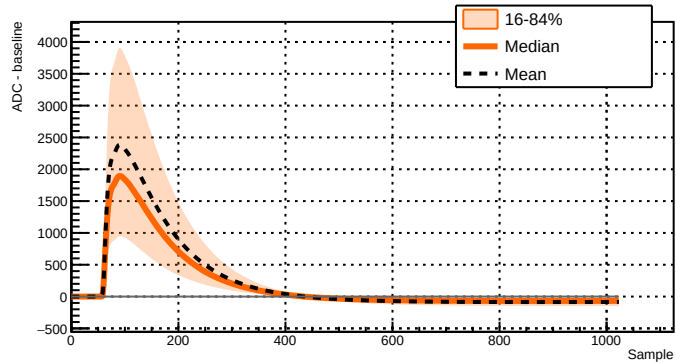
Run 039507 - Channel 2081 - 22652 waveforms
