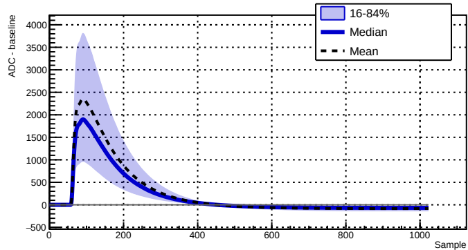
Run 039517 - Channel 2080 - 20444 waveforms
