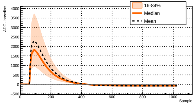
Run 039517 - Channel 2081 - 20978 waveforms
