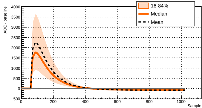
Run 039518 - Channel 2081 - 20472 waveforms
