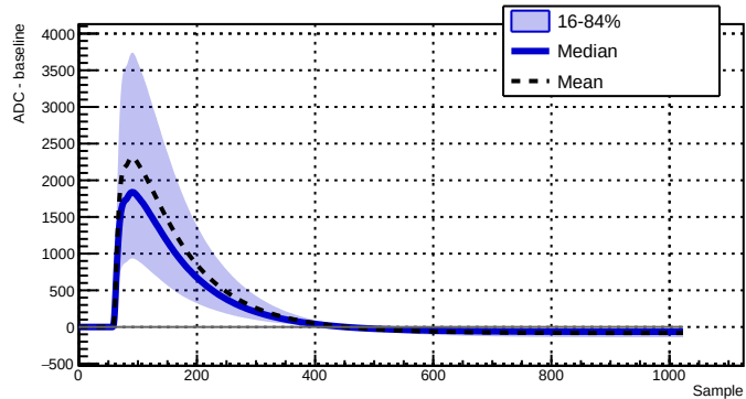
Run 039518 - Channel 2080 - 19885 waveforms
