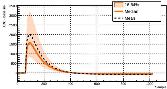
Run 039526 - Channel 2081 - 17499 waveforms
