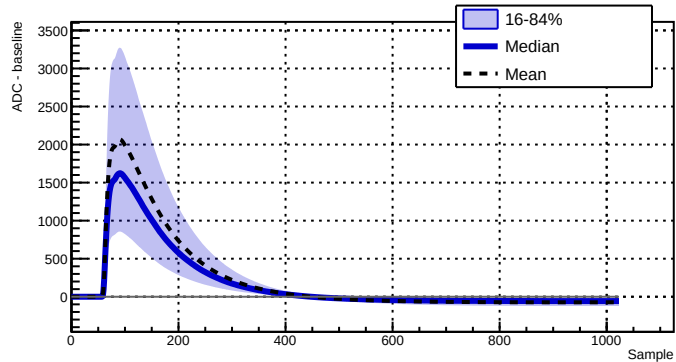
Run 039526 - Channel 2080 - 17091 waveforms
