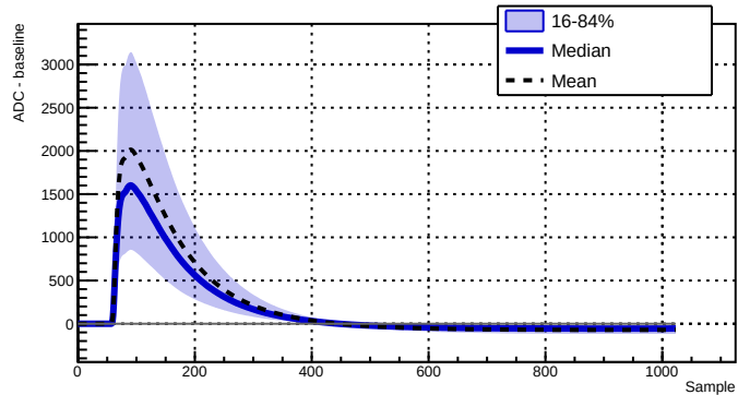
Run 039528 - Channel 2080 - 16418 waveforms
