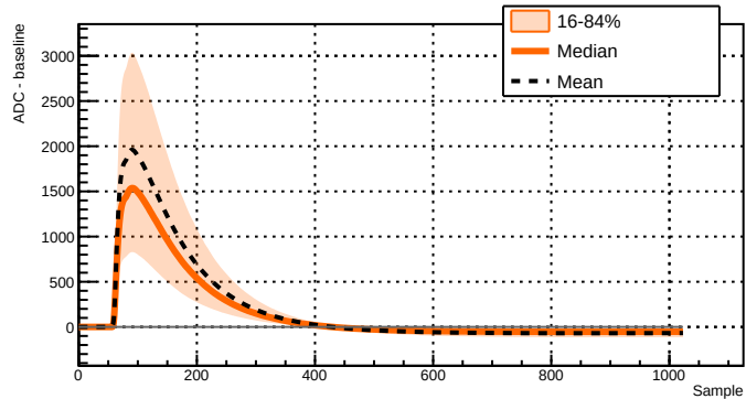
Run 039528 - Channel 2081 - 16904 waveforms
