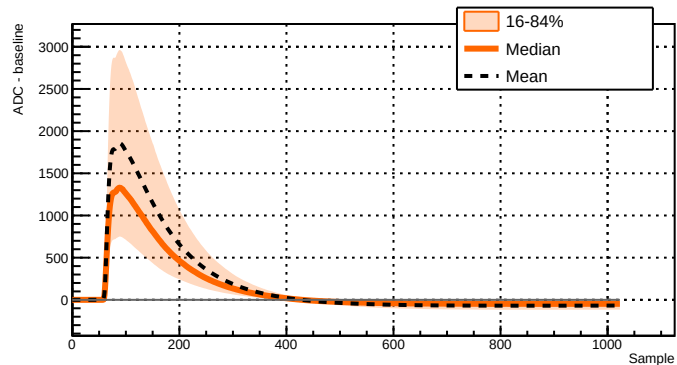
Run 039500 - Channel 2051 - 10897 waveforms
