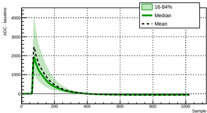
Run 039500 - Channel 2060 - 12363 waveforms
