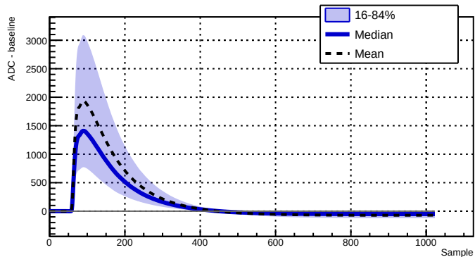
Run 039500 - Channel 2050 - 16986 waveforms
