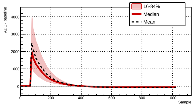
Run 039500 - Channel 2061 - 7932 waveforms
