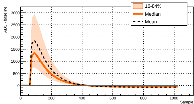
Run 039501 - Channel 2051 - 11339 waveforms
