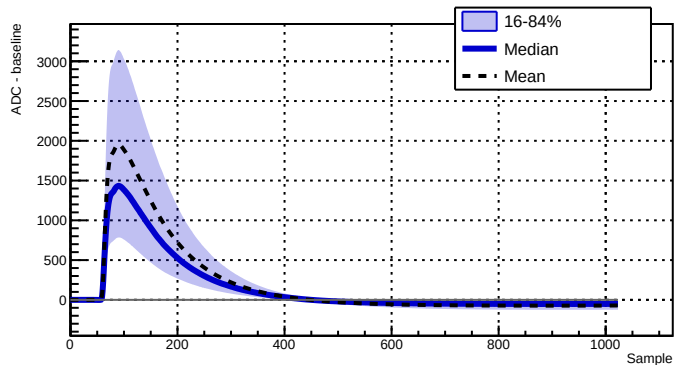
Run 039501 - Channel 2050 - 17635 waveforms
