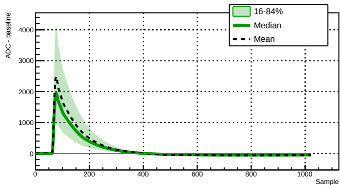
Run 039501 - Channel 2060 - 12760 waveforms
