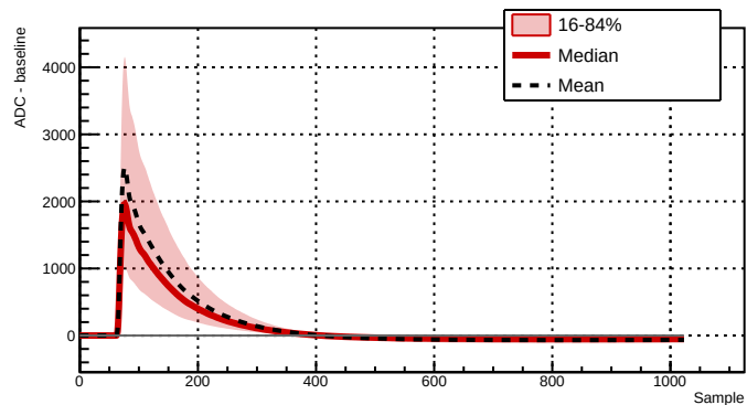
Run 039501 - Channel 2061 - 8222 waveforms
