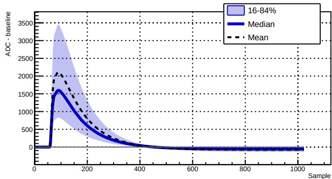
Run 039504 - Channel 2050 - 20076 waveforms
