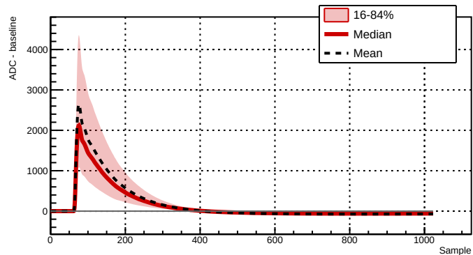
Run 039504 - Channel 2061 - 9749 waveforms
