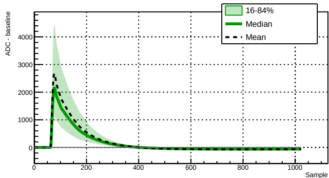
Run 039504 - Channel 2060 - 14614 waveforms
