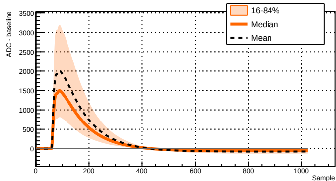
Run 039504 - Channel 2051 - 13201 waveforms
