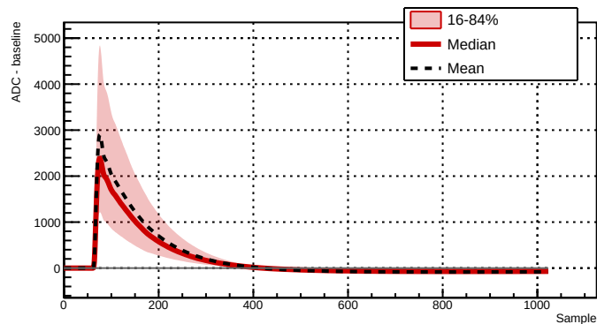
Run 039508 - Channel 2061 - 11015 waveforms
