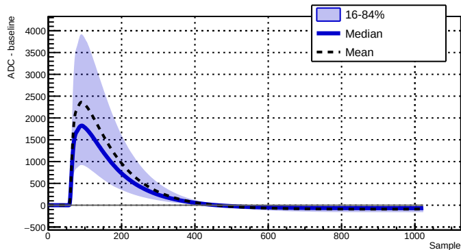
Run 039508 - Channel 2050 - 23113 waveforms
