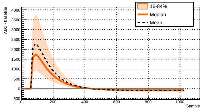
Run 039508 - Channel 2051 - 15555 waveforms
