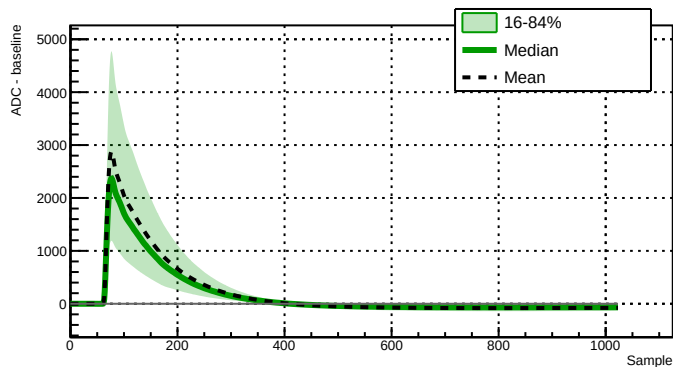
Run 039508 - Channel 2060 - 16689 waveforms
