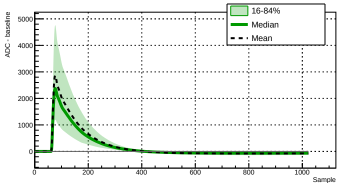
Run 039512 - Channel 2060 - 16894 waveforms
