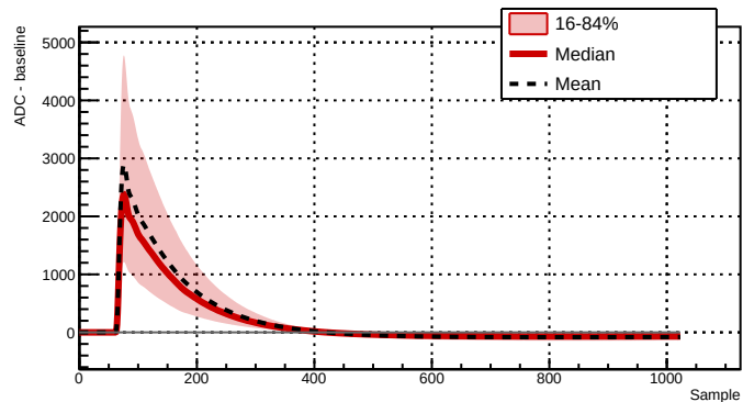
Run 039512 - Channel 2061 - 11195 waveforms
