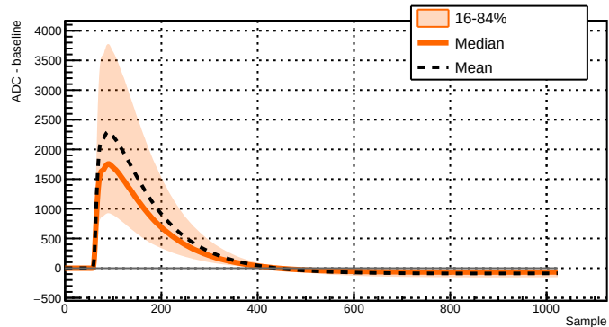
Run 039512 - Channel 2051 - 15880 waveforms
