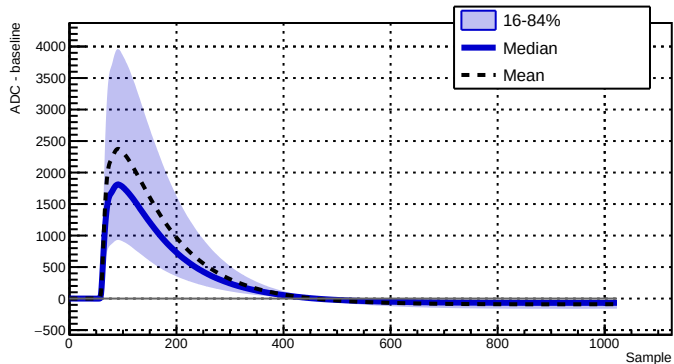
Run 039512 - Channel 2050 - 23350 waveforms
