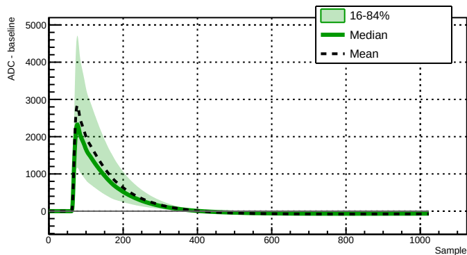
Run 039514 - Channel 2060 - 16252 waveforms
