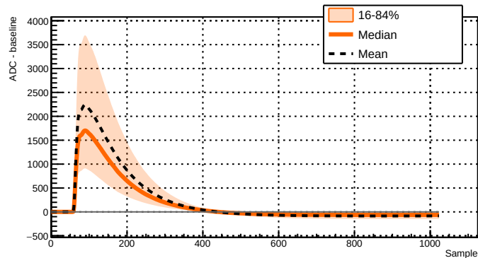
Run 039514 - Channel 2051 - 15059 waveforms
