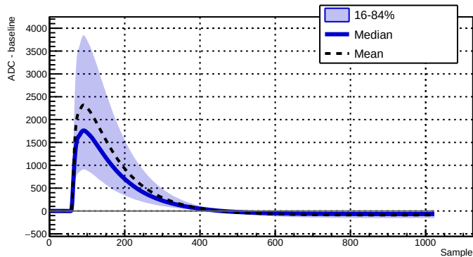
Run 039514 - Channel 2050 - 22642 waveforms
