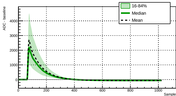
Run 039518 - Channel 2060 - 14872 waveforms
