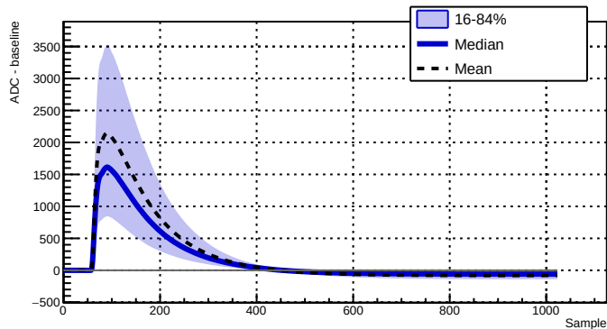
Run 039518 - Channel 2050 - 20417 waveforms
