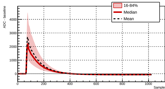
Run 039518 - Channel 2061 - 9717 waveforms
