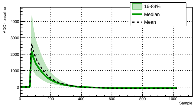
Run 039519 - Channel 2060 - 14406 waveforms
