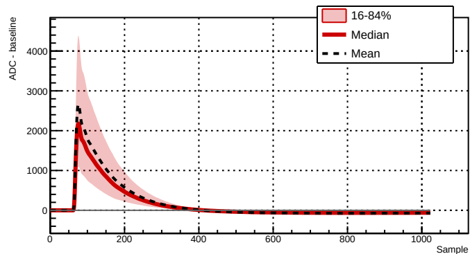
Run 039519 - Channel 2061 - 9442 waveforms
