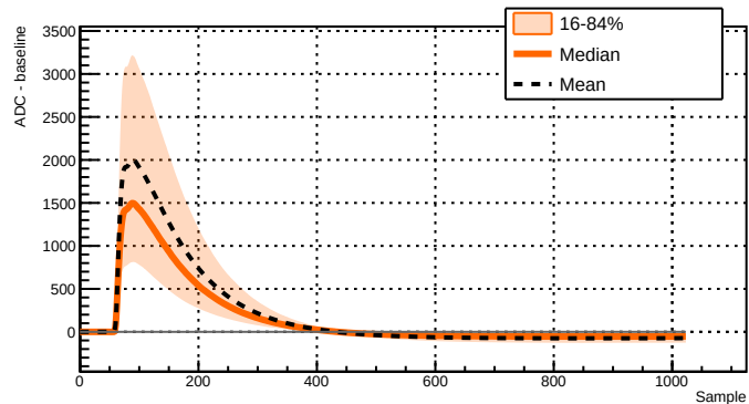
Run 039519 - Channel 2051 - 12985 waveforms
