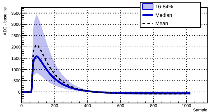
Run 039519 - Channel 2050 - 19955 waveforms
