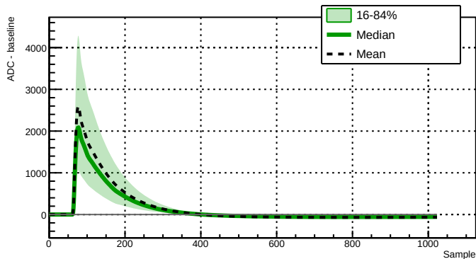
Run 039521 - Channel 2060 - 13825 waveforms
