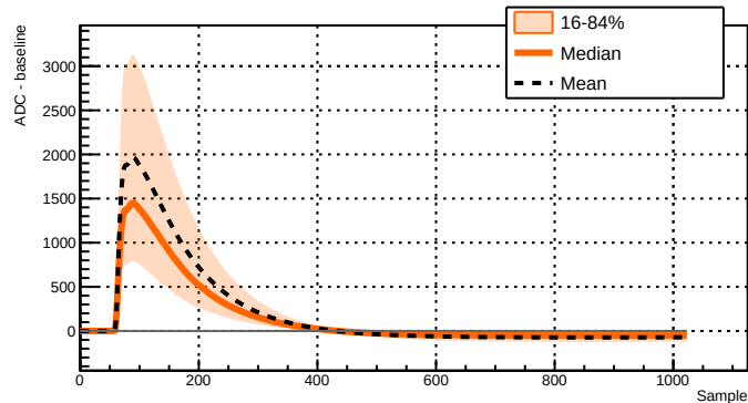
Run 039521 - Channel 2051 - 12377 waveforms
