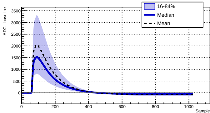
Run 039521 - Channel 2050 - 19310 waveforms
