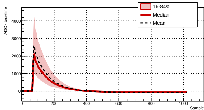
Run 039521 - Channel 2061 - 8950 waveforms
