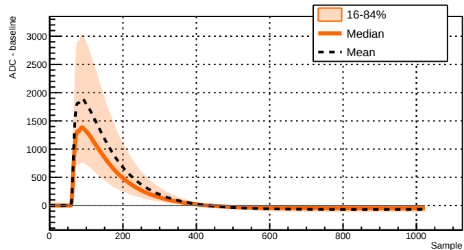
Run 039526 - Channel 2051 - 11167 waveforms
