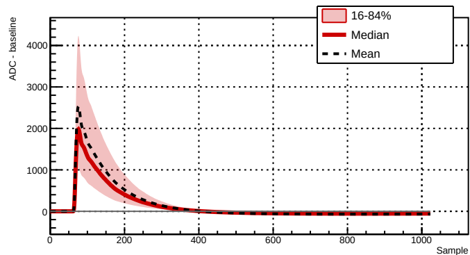
Run 039526 - Channel 2061 - 8187 waveforms
