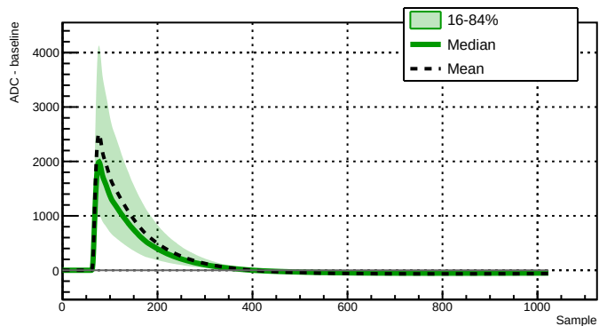
Run 039526 - Channel 2060 - 12671 waveforms
