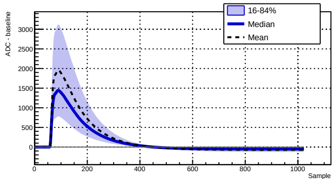
Run 039526 - Channel 2050 - 17801 waveforms
