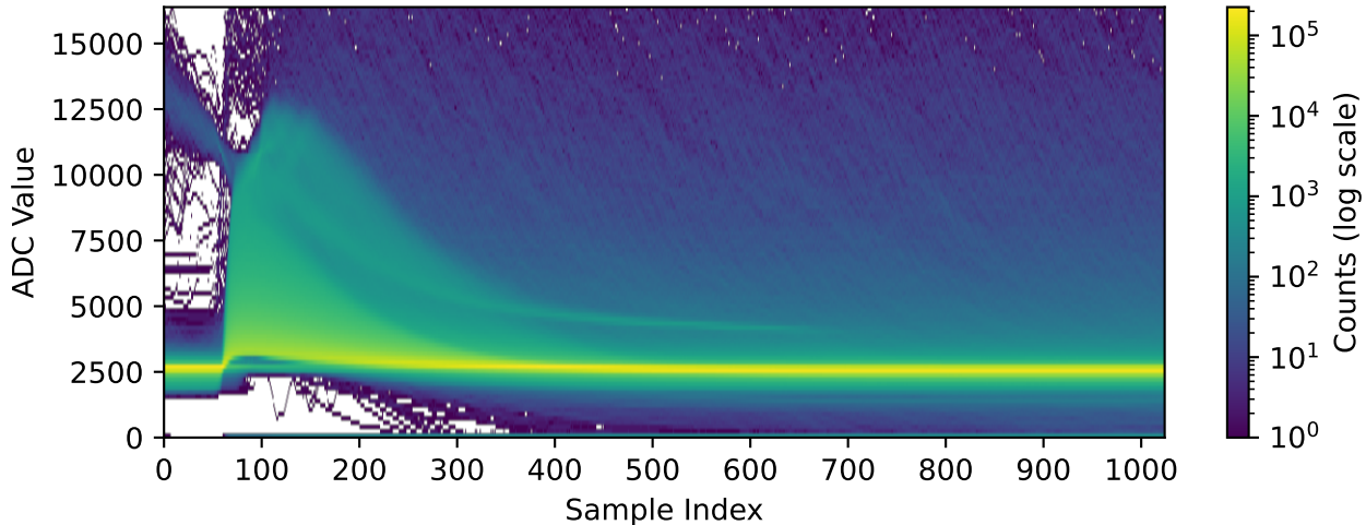
Channel 2031 (n=286613 waveforms)
