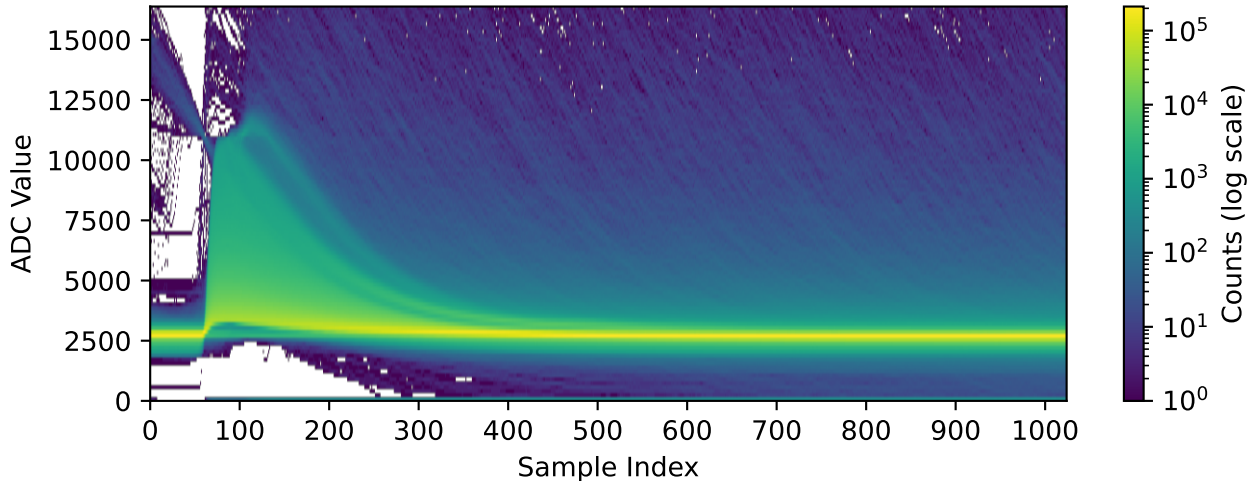
Channel 2040 (n=297634 waveforms)
