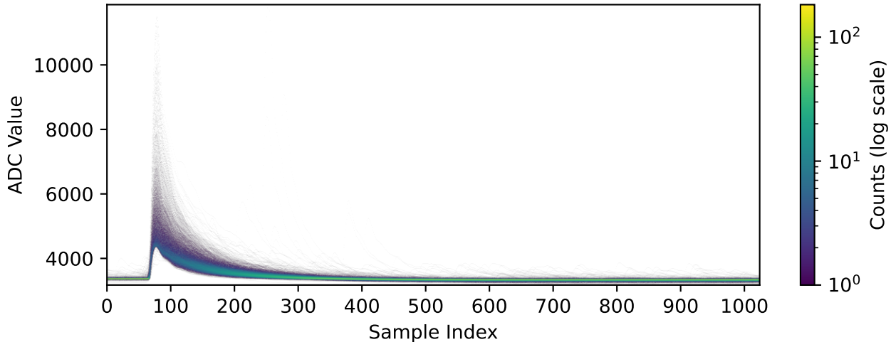
Channel 2070 (n=3268 waveforms)
