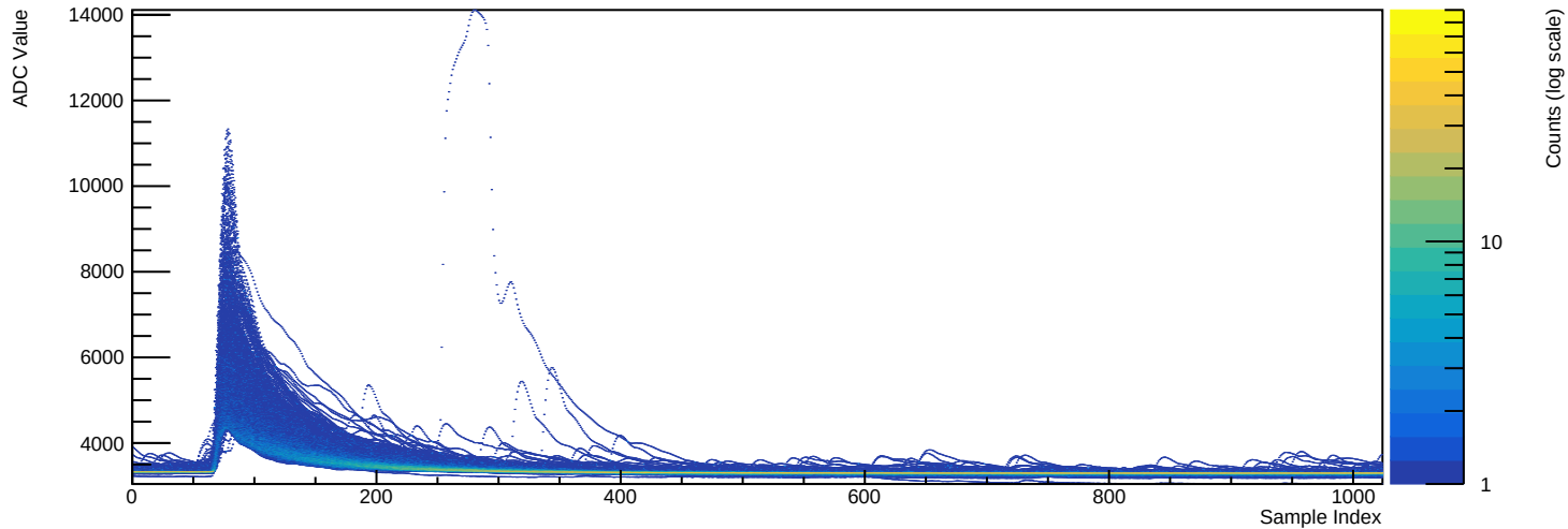
Run 039502 - Channel 2070 (n=1415 waveforms)
