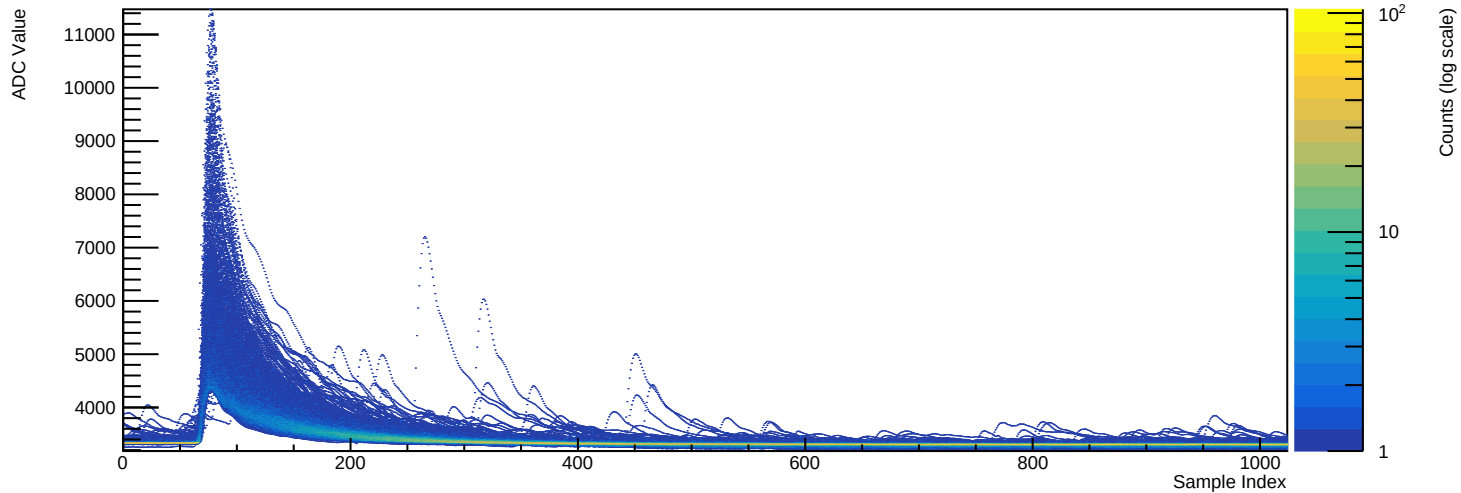
Run 039503 - Channel 2070 (n=1548 waveforms)
