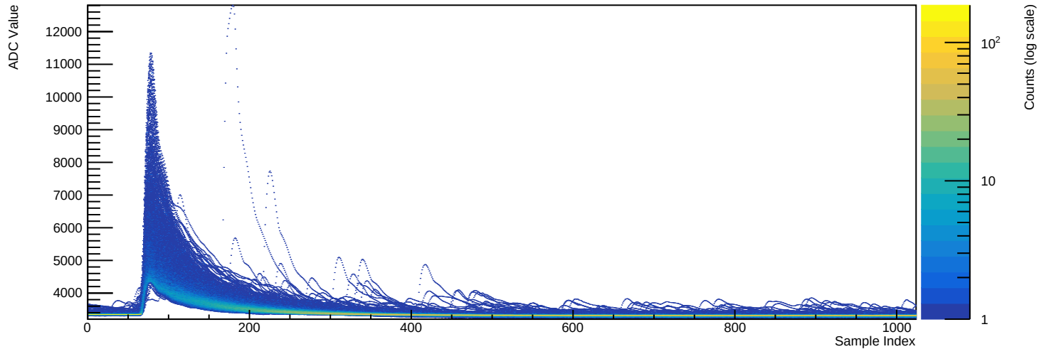
Run 039508 - Channel 2070 (n=2746 waveforms)
