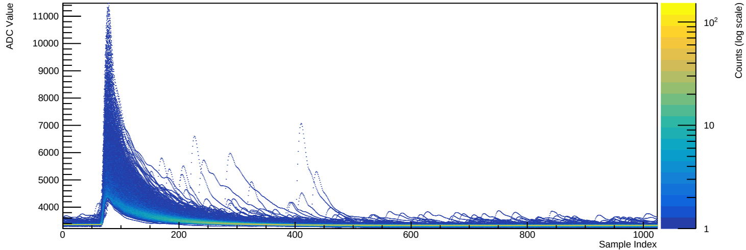
Run 039515 - Channel 2070 (n=2272 waveforms)
