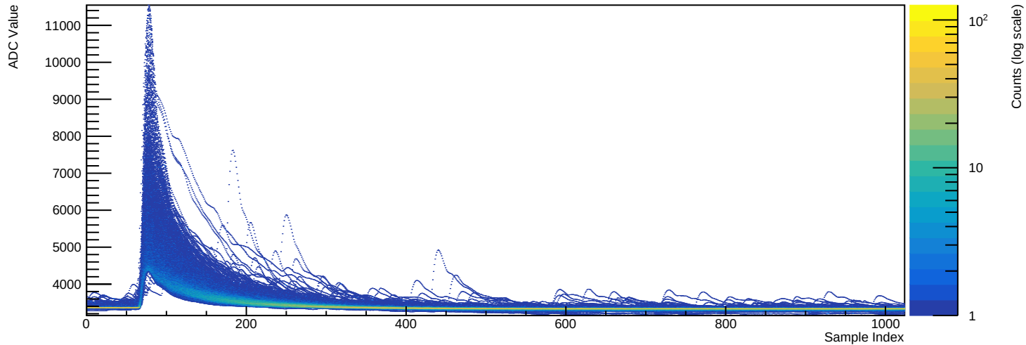
Run 039517 - Channel 2070 (n=1948 waveforms)
