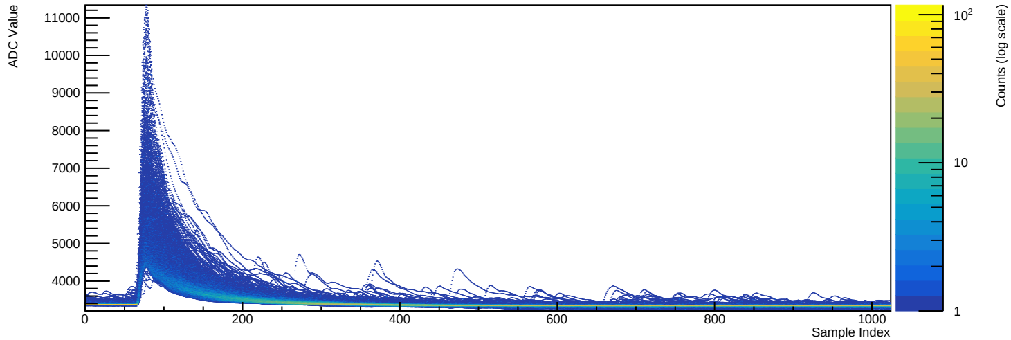
Run 039521 - Channel 2070 (n=1538 waveforms)
