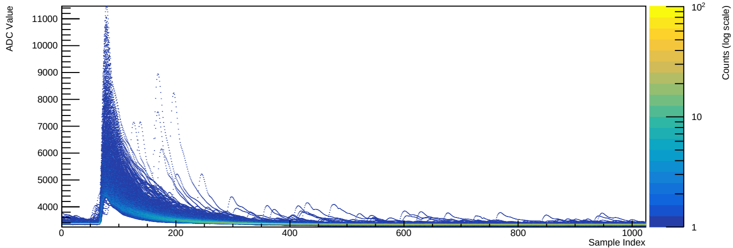
Run 039523 - Channel 2070 (n=1412 waveforms)
