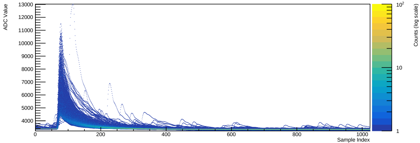
Run 039525 - Channel 2070 (n=1344 waveforms)
