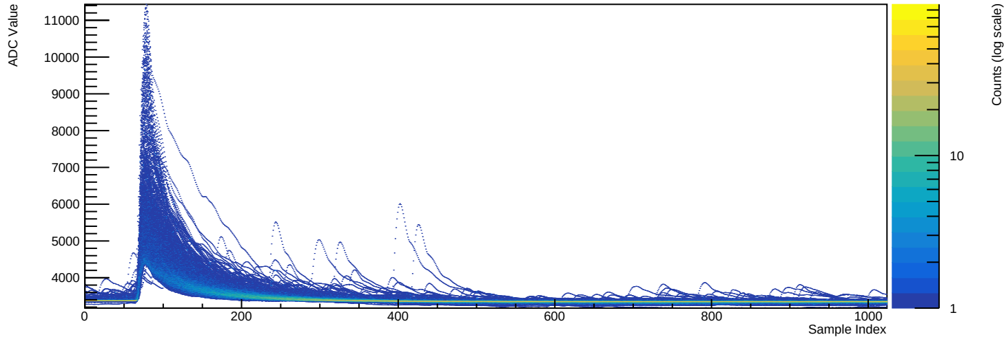
Run 039527 - Channel 2070 (n=1260 waveforms)
