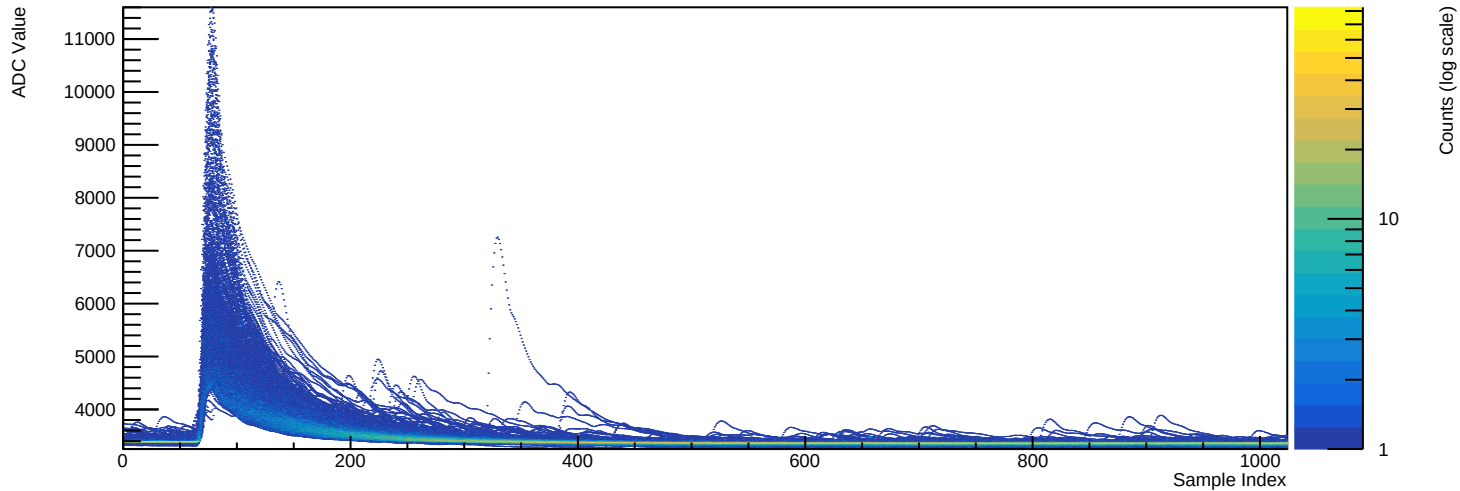
Run 039501 - Channel 2071 (n=1199 waveforms)
