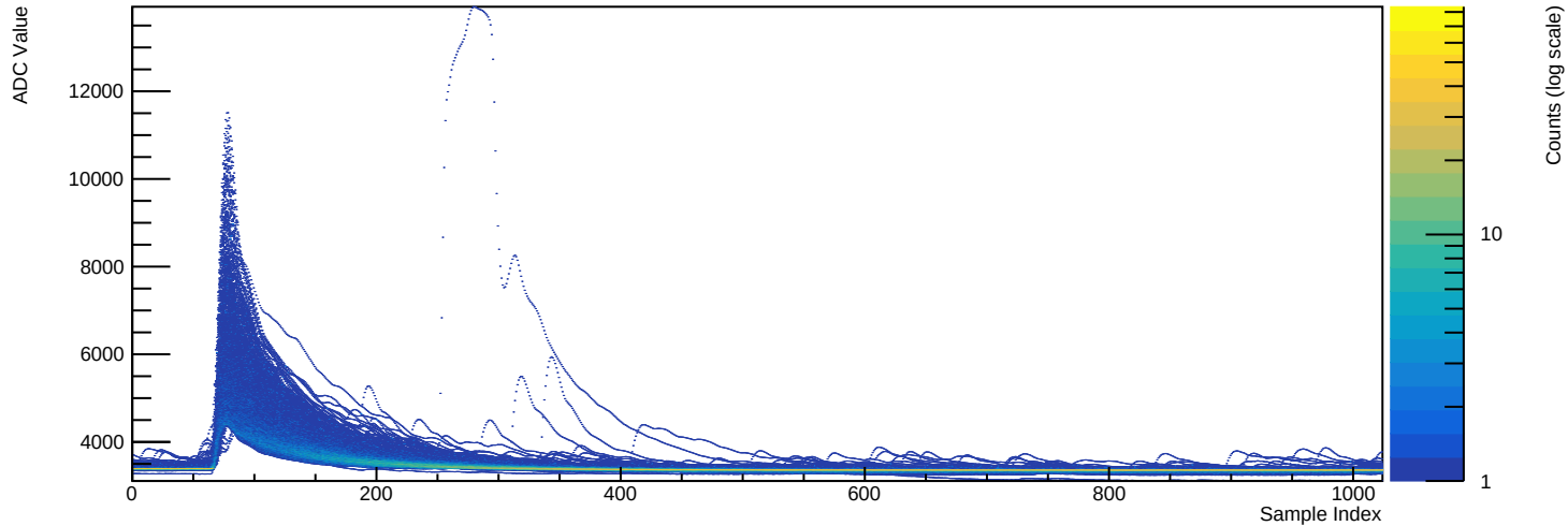
Run 039502 - Channel 2071 (n=1326 waveforms)
