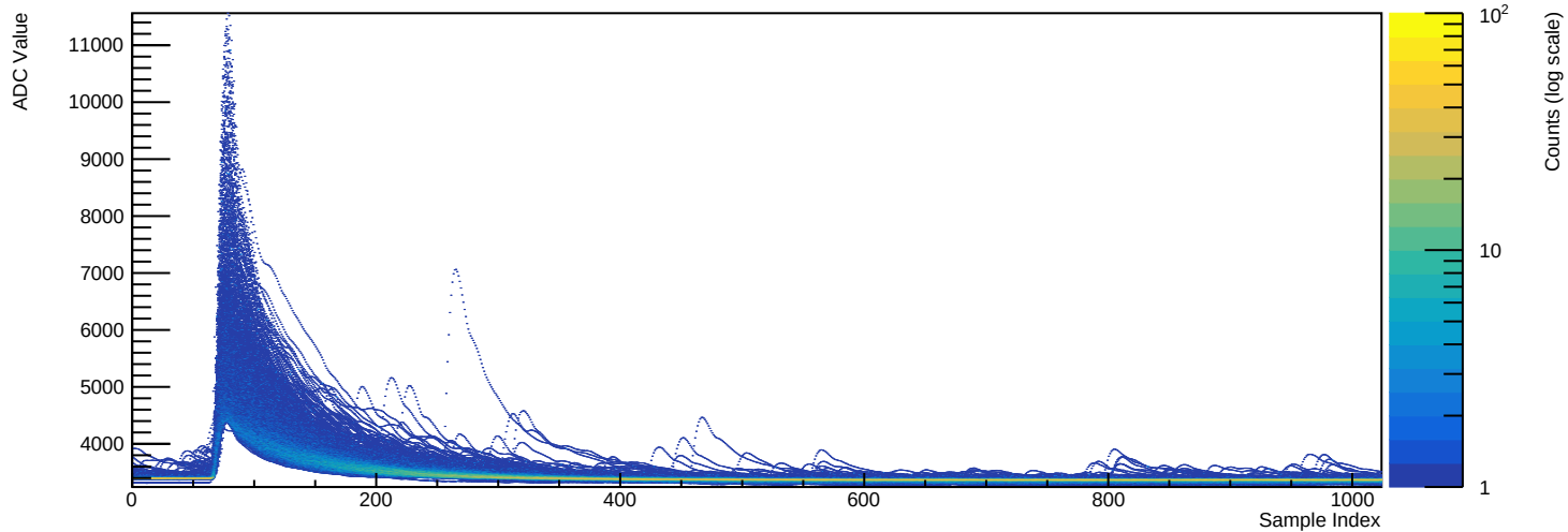
Run 039503 - Channel 2071 (n=1462 waveforms)
