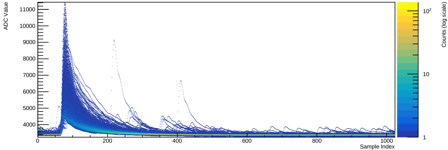
Run 039507 - Channel 2071 (n=2069 waveforms)
