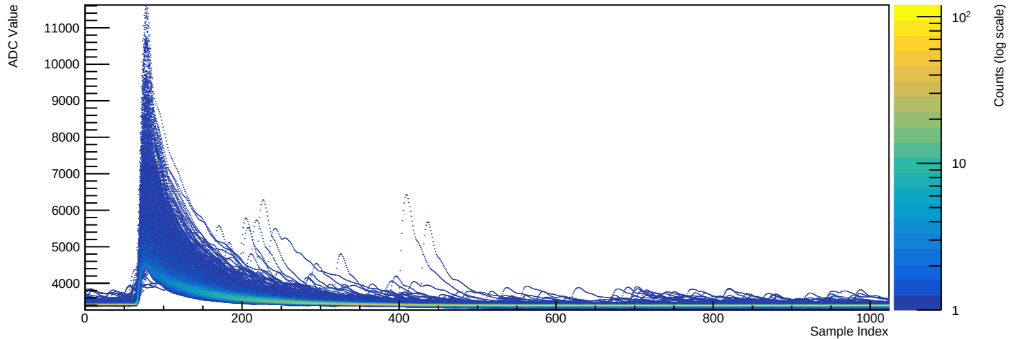
Run 039515 - Channel 2071 (n=2131 waveforms)
