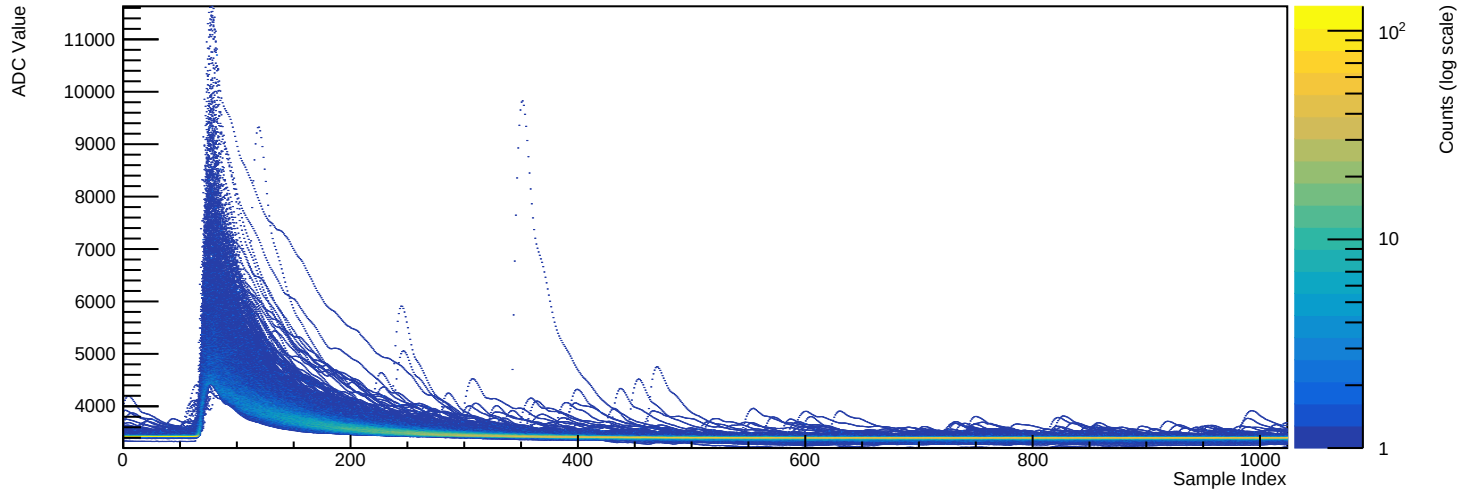
Run 039516 - Channel 2071 (n=1940 waveforms)
