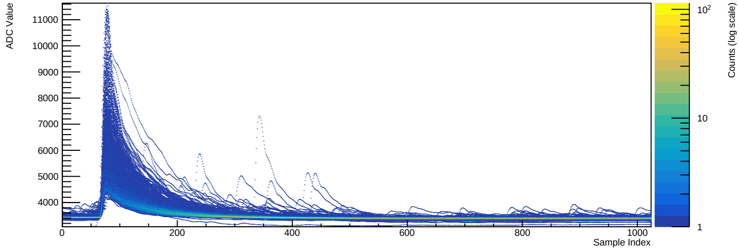
Run 039519 - Channel 2071 (n=1598 waveforms)
