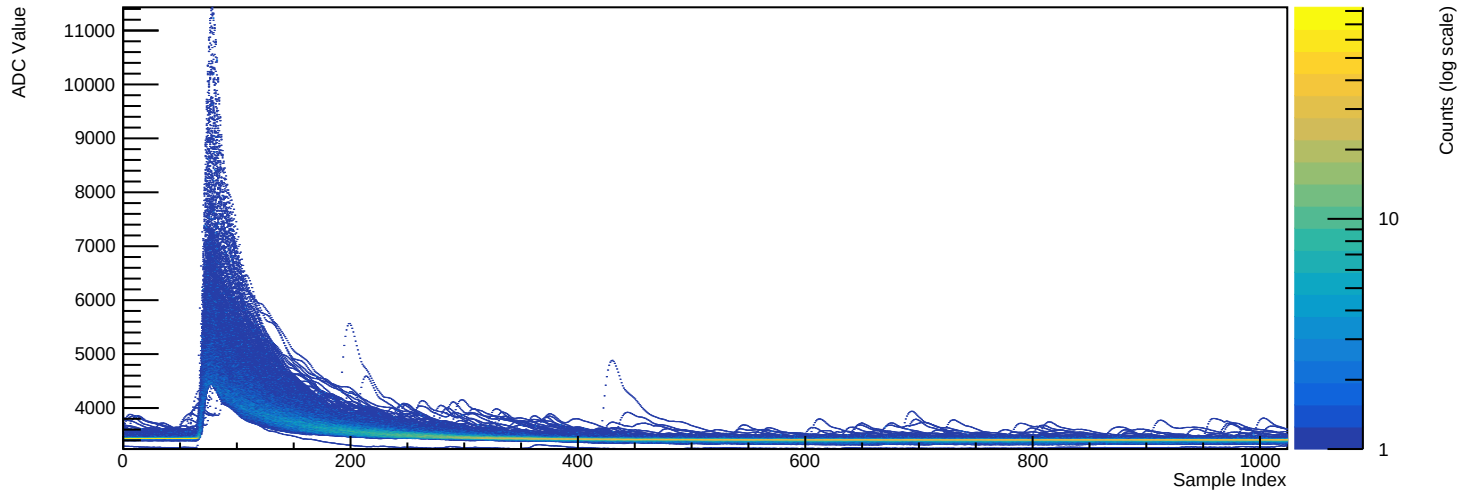
Run 039526 - Channel 2071 (n=1225 waveforms)
